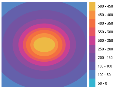
Prime Full Power @ 47W Standard 80° Lens - 18" x 18" - 12" Height μMol Units
